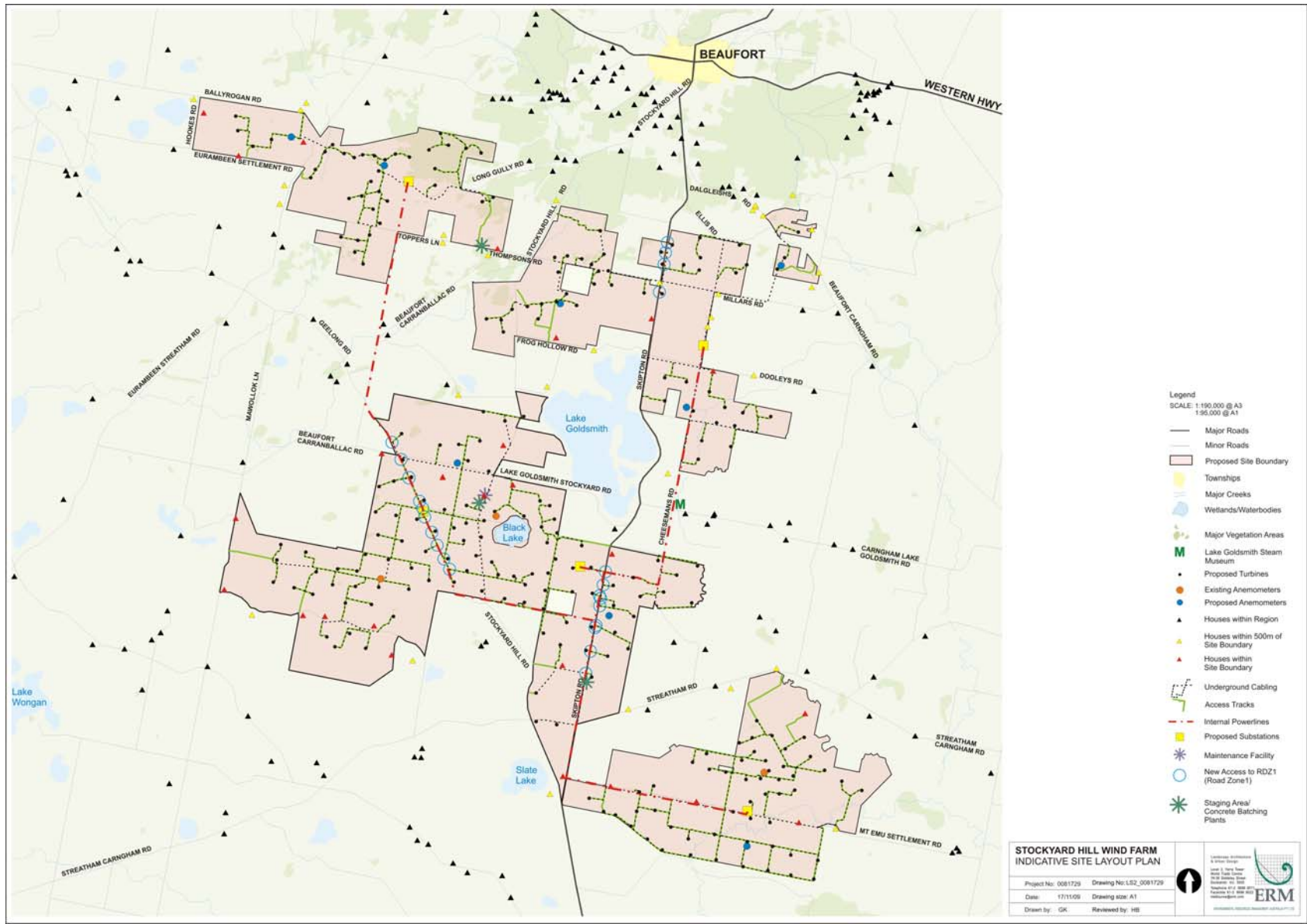
Figure 4.1 Indicative Site Layout Plan
